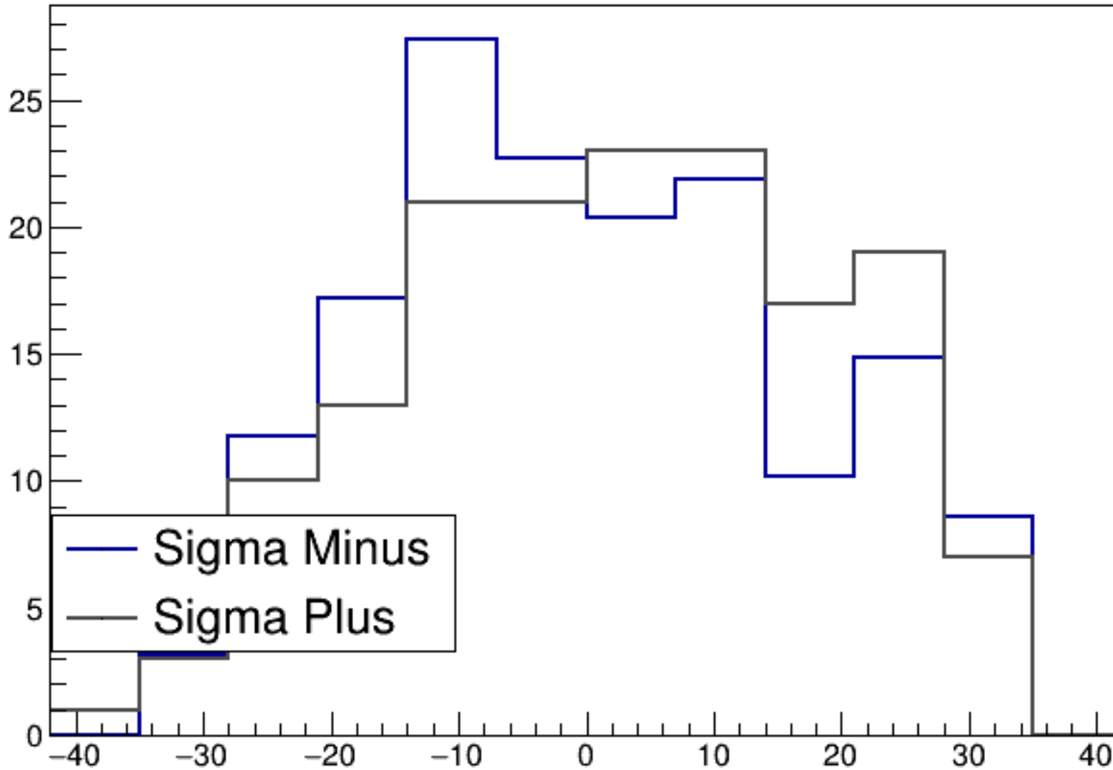
Histogram showing Sigma Plus and Sigma Minus Z position distributions on ION MCP(mm)
